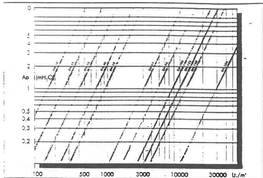
Loss of head diagram
